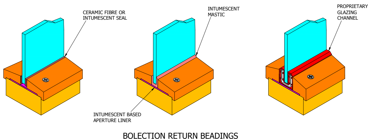
Diagram 6 – Examples of 60 minute timber framing details
